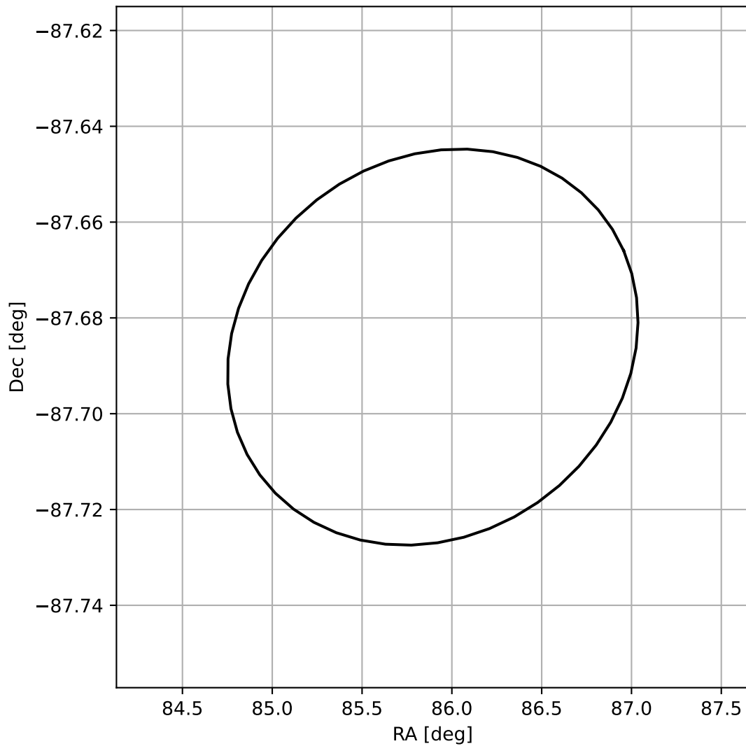
4FGL J0543.5-8741
