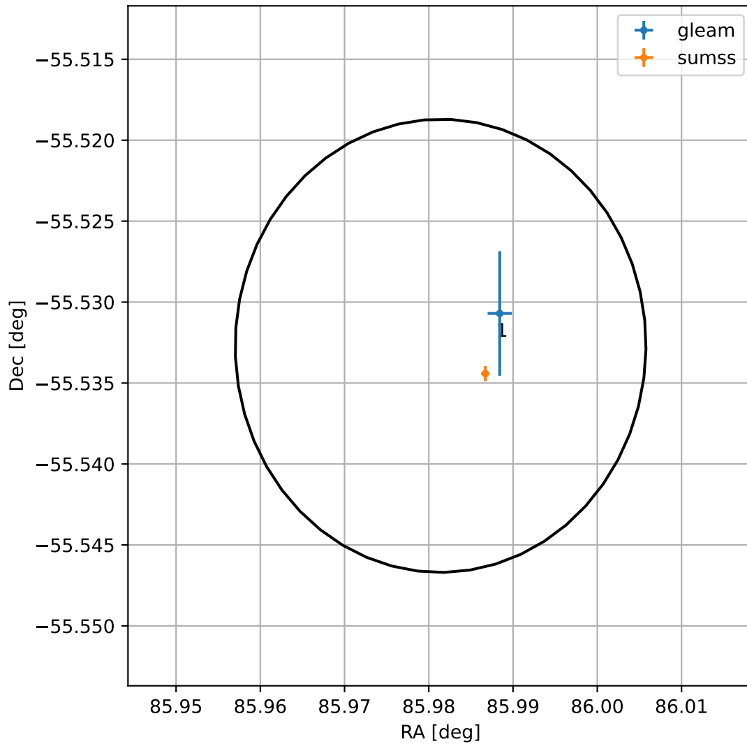
4FGL J0543.9-5531
