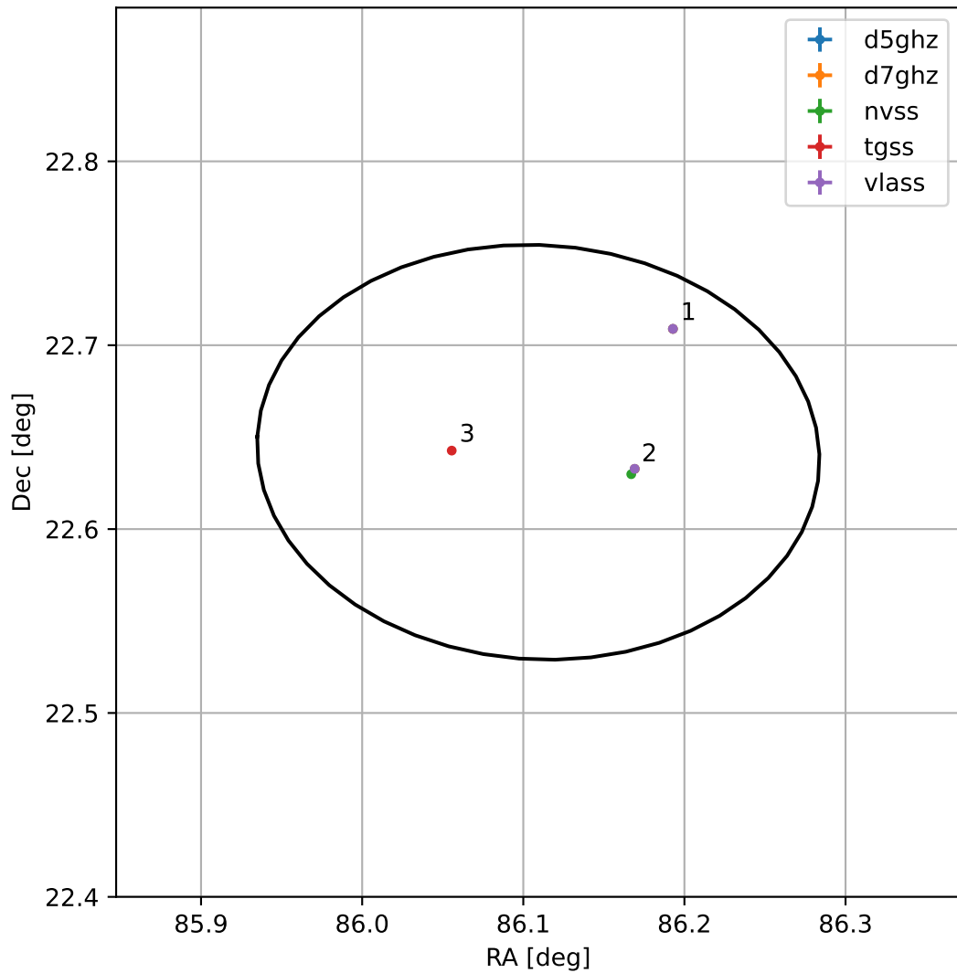
4FGL J0544.4+2238
