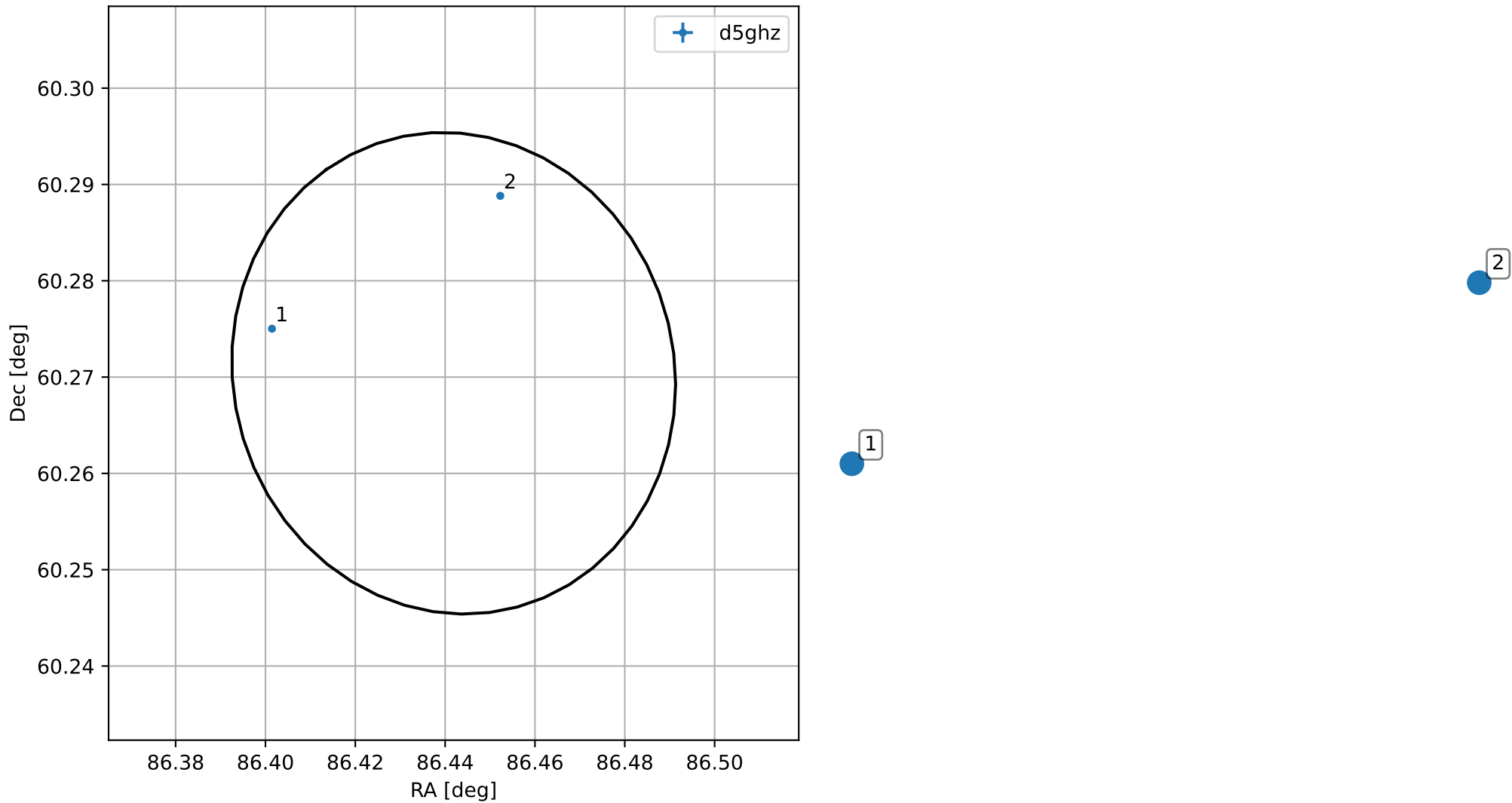
4FGL J0545.7+6016
