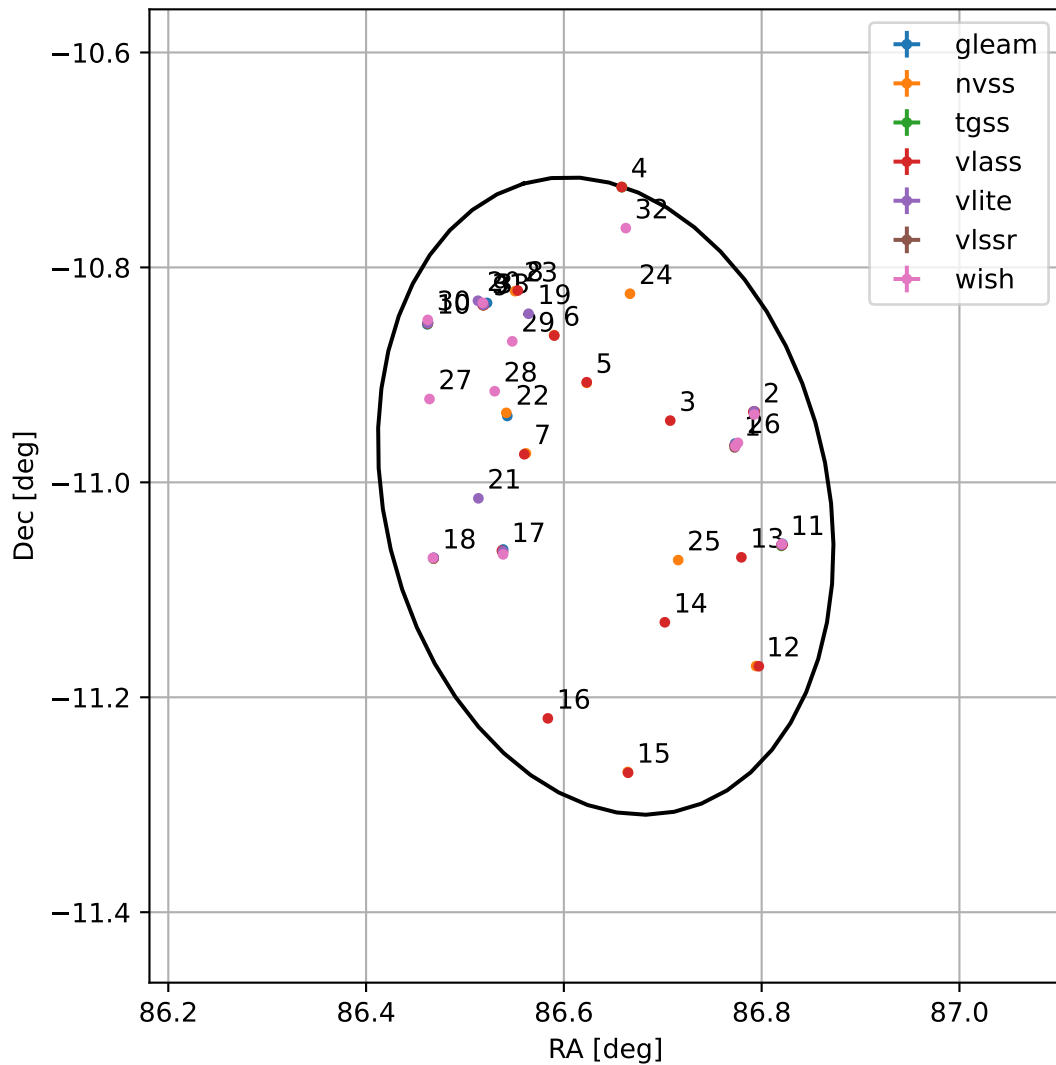
4FGL J0546.5-1100
