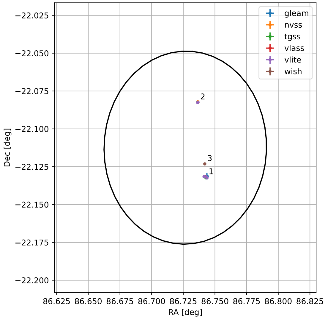
4FGL J0546.9-2206
