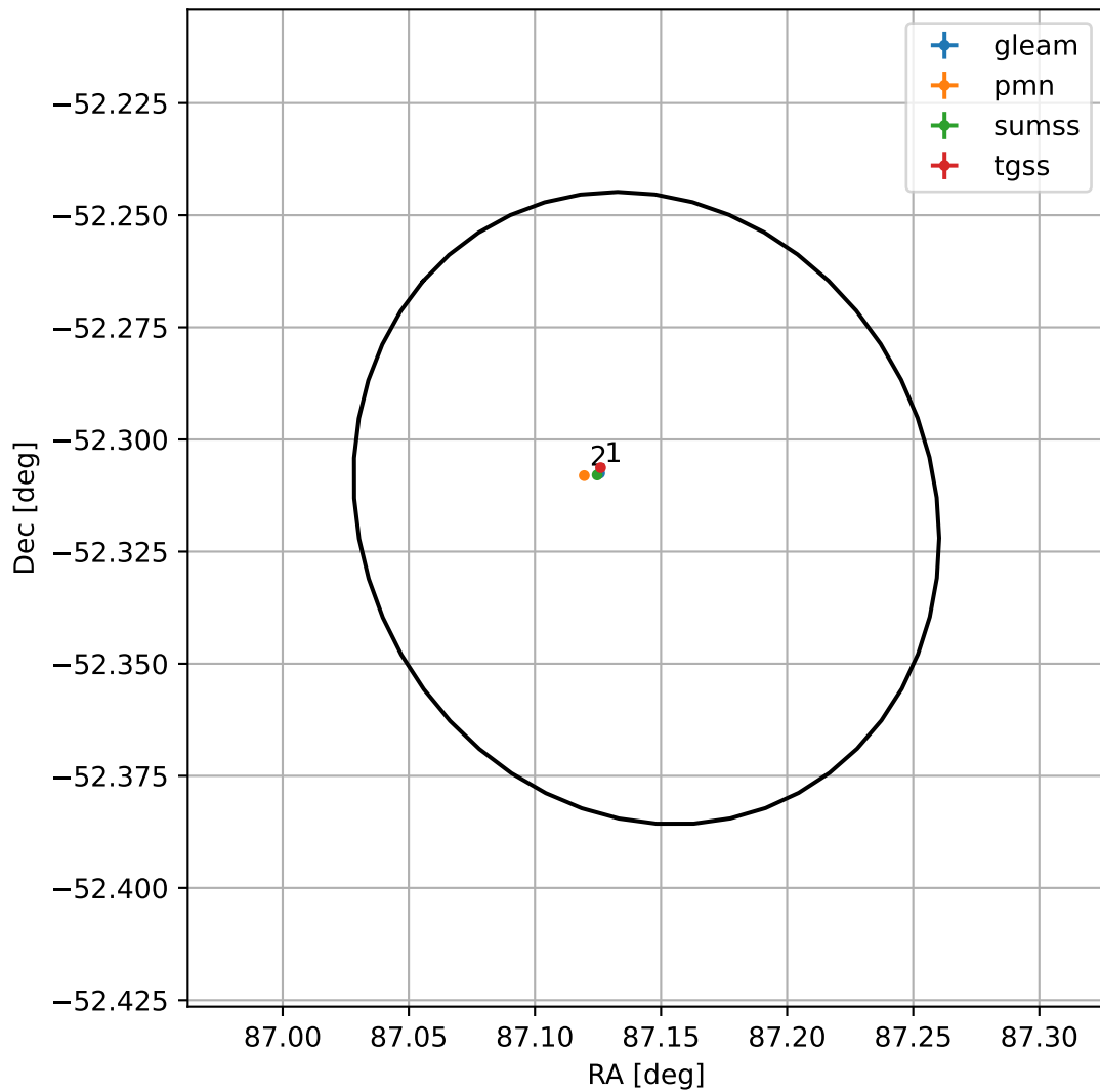
4FGL J0548.5-5218
