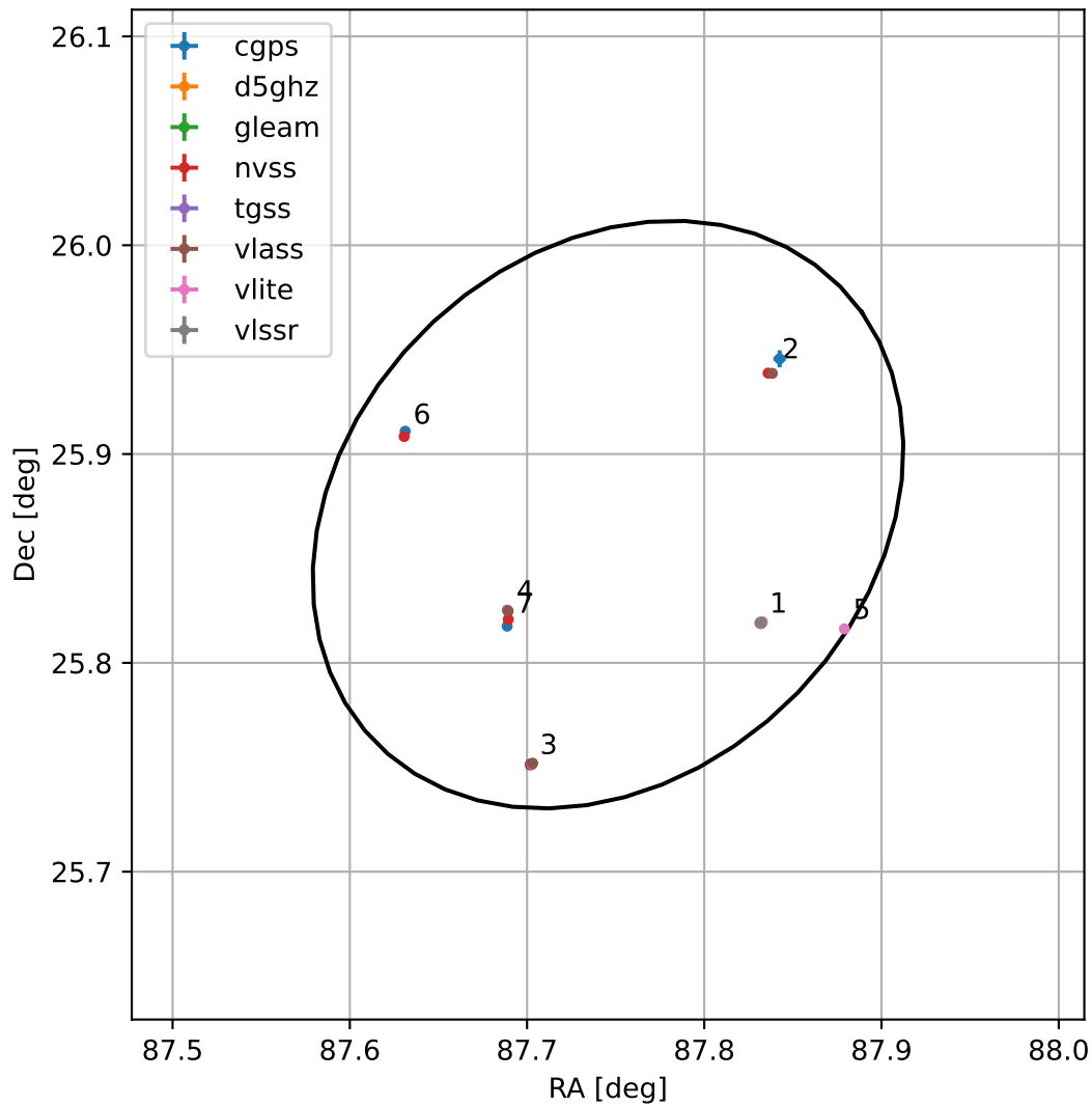
4FGL J0550.9+2552
