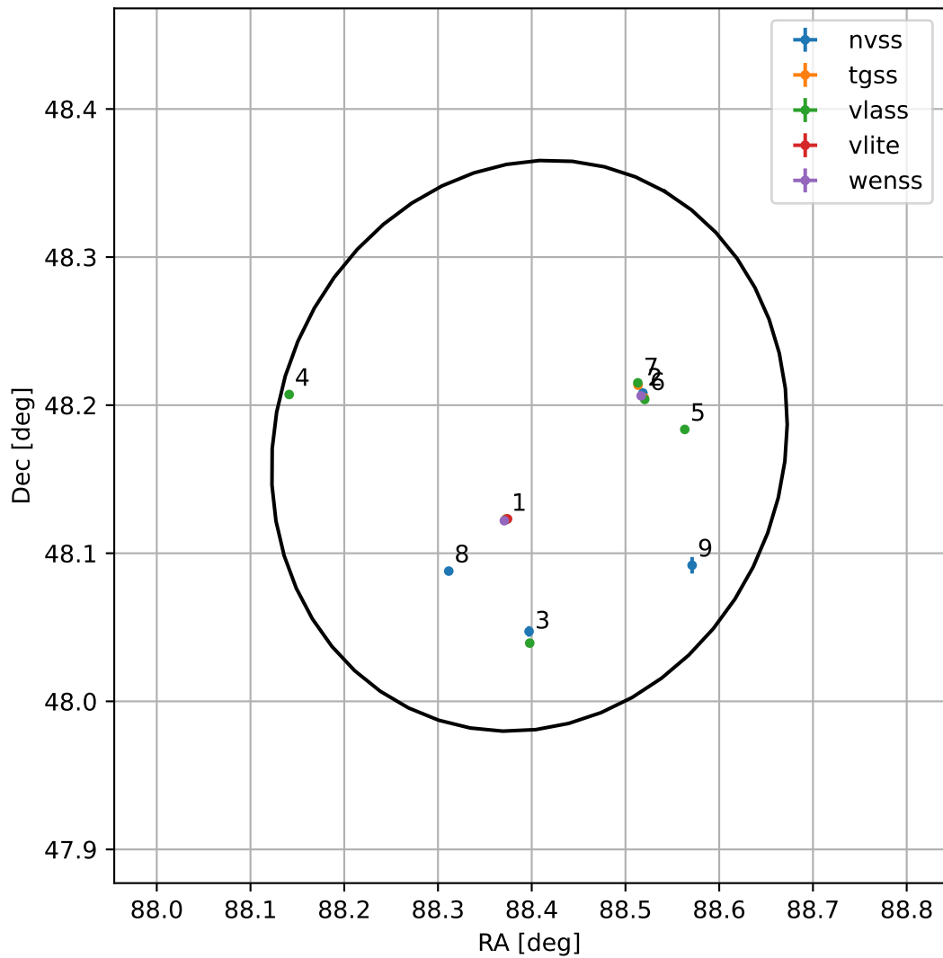
4FGL J0553.5+4810
