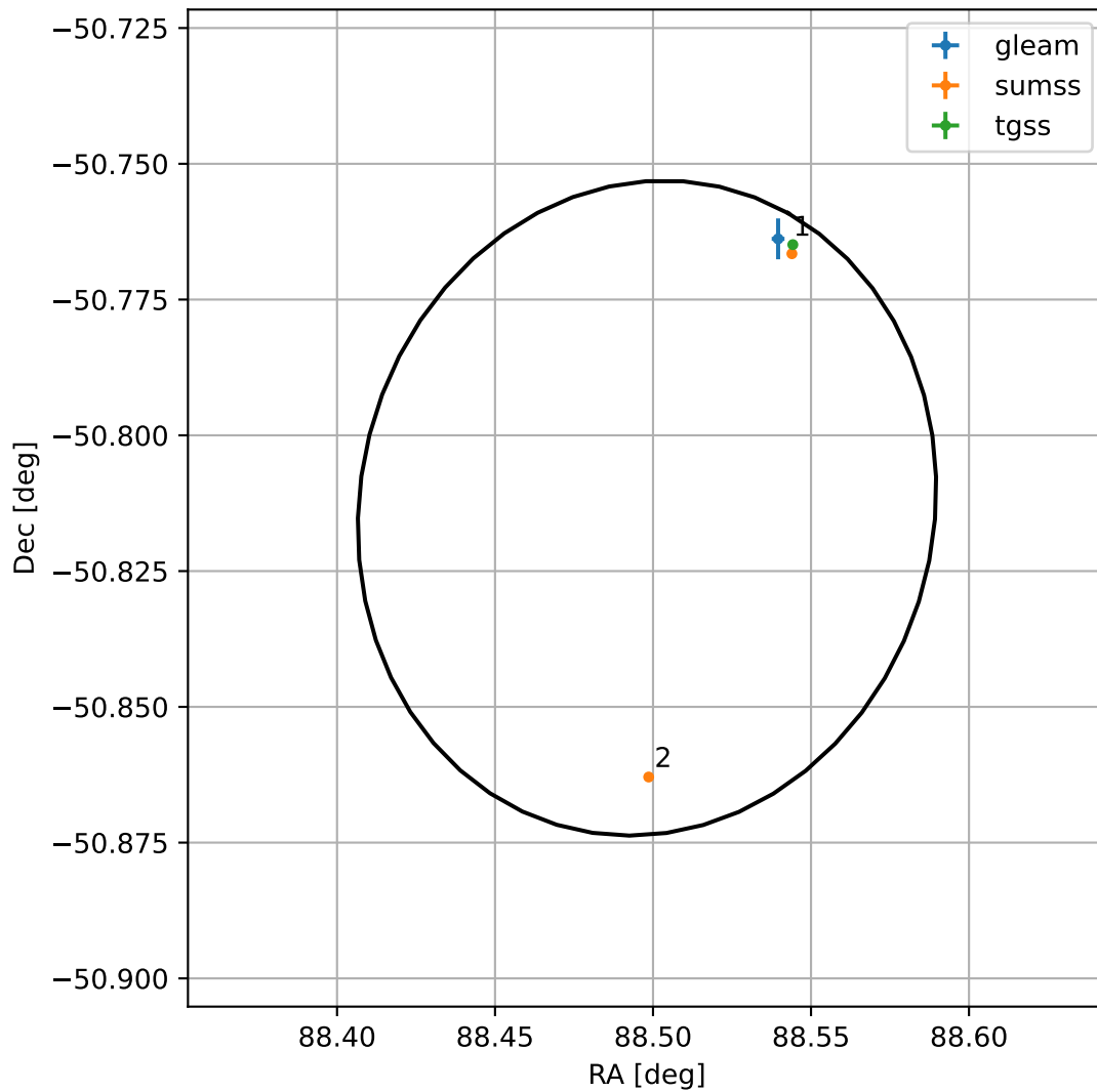
4FGL J0553.9-5048
