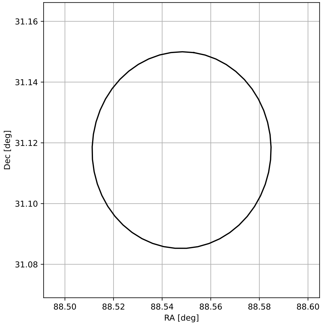
4FGL J0554.1+3107
