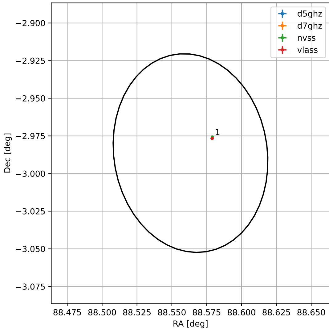
4FGL J0554.2-0259
