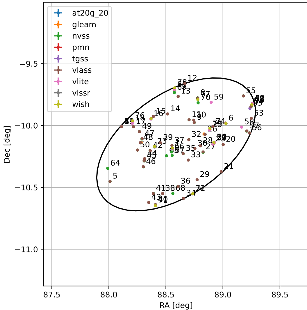
4FGL J0554.3-1009
