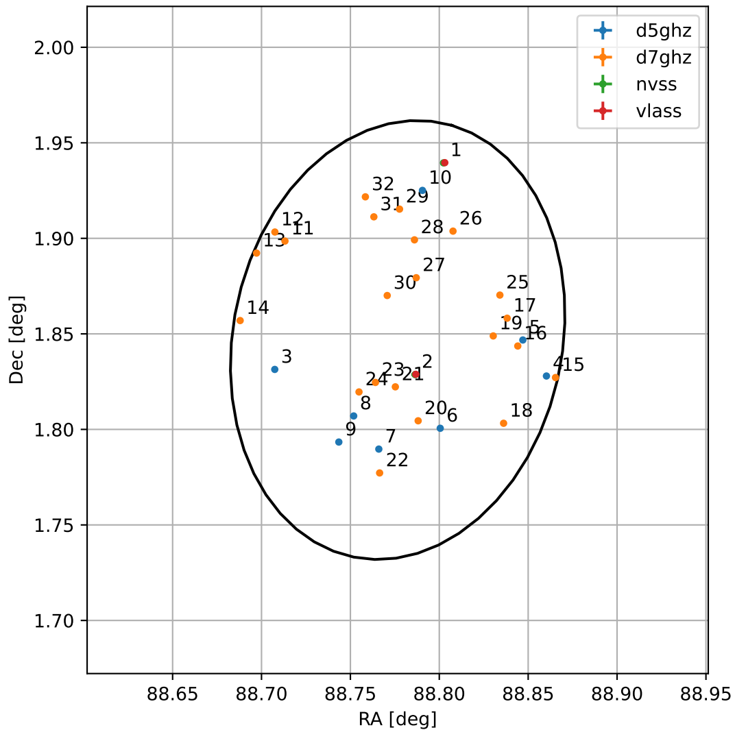
4FGL J0555.1+0150
