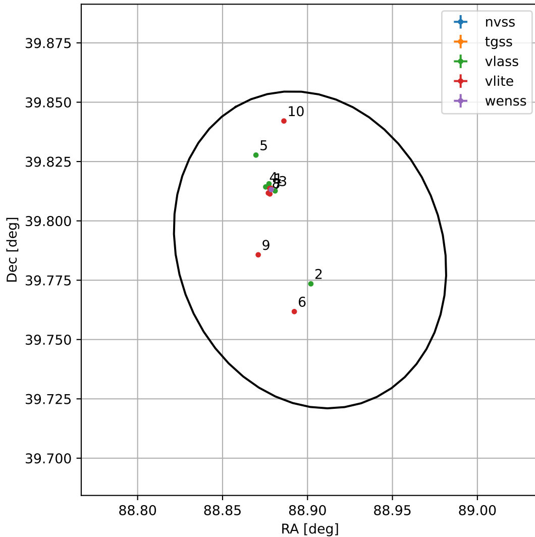
4FGL J0555.6+3947
