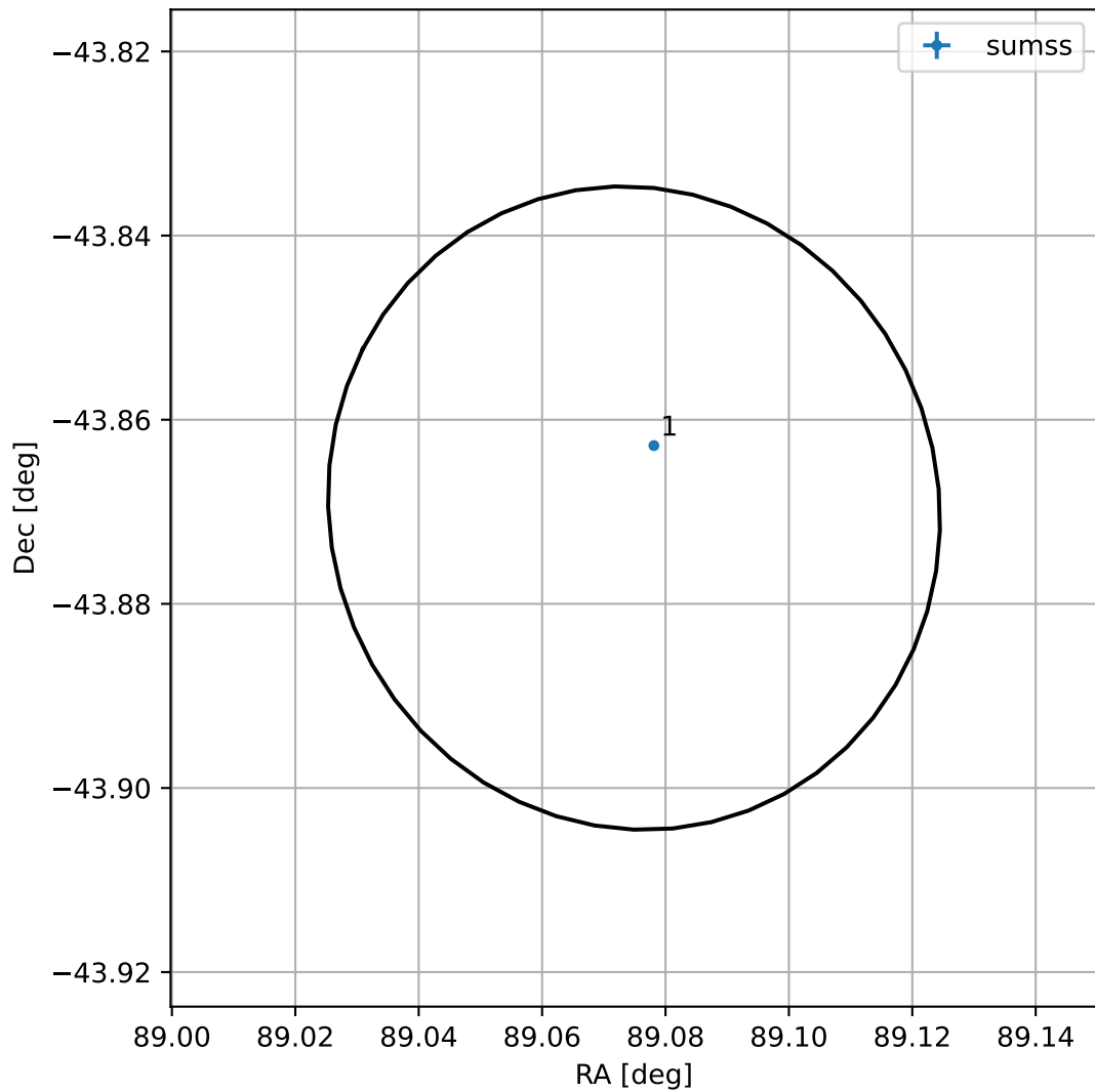
4FGL J0556.2-4352
