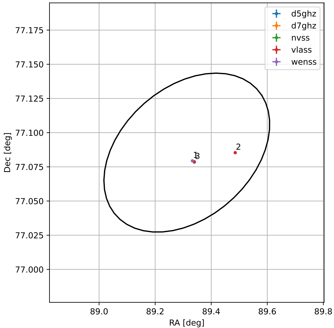
4FGL J0557.2+7705
