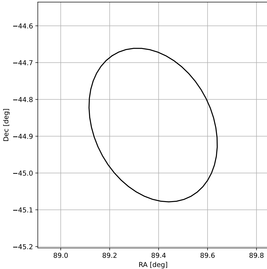
4FGL J0557.5-4452
