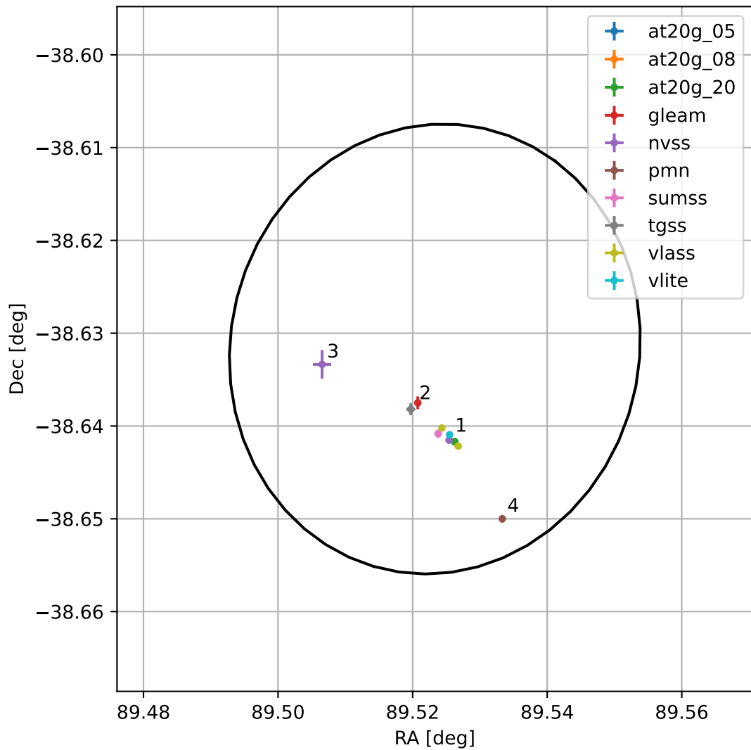
4FGL J0558.0-3837
