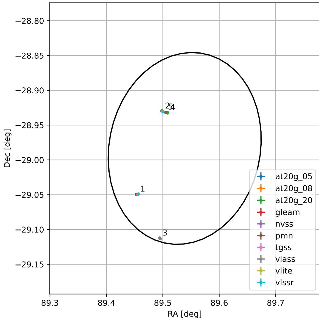
4FGL J0558.1-2859
