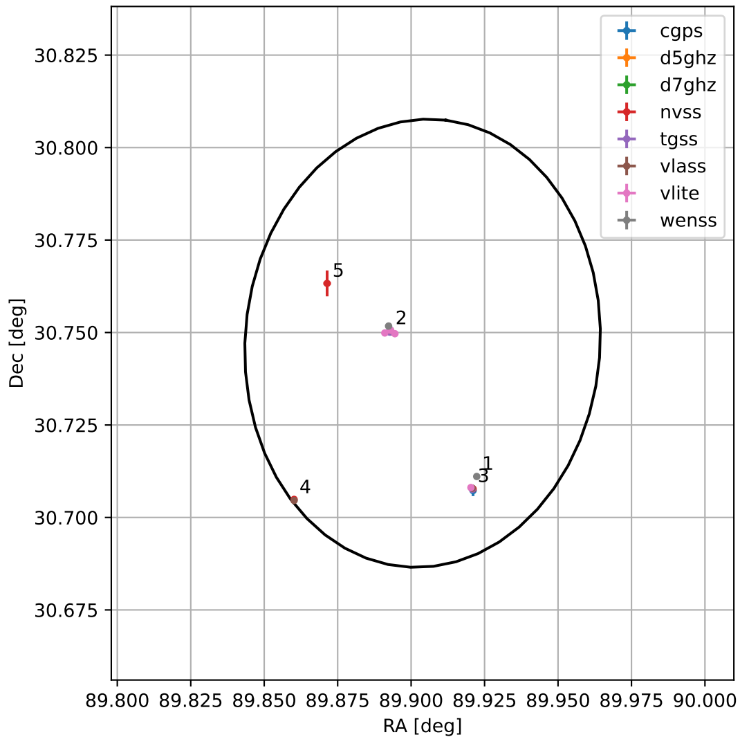
4FGL J0559.6+3044
