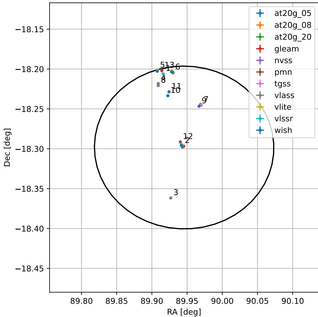
4FGL J0559.7-1817
