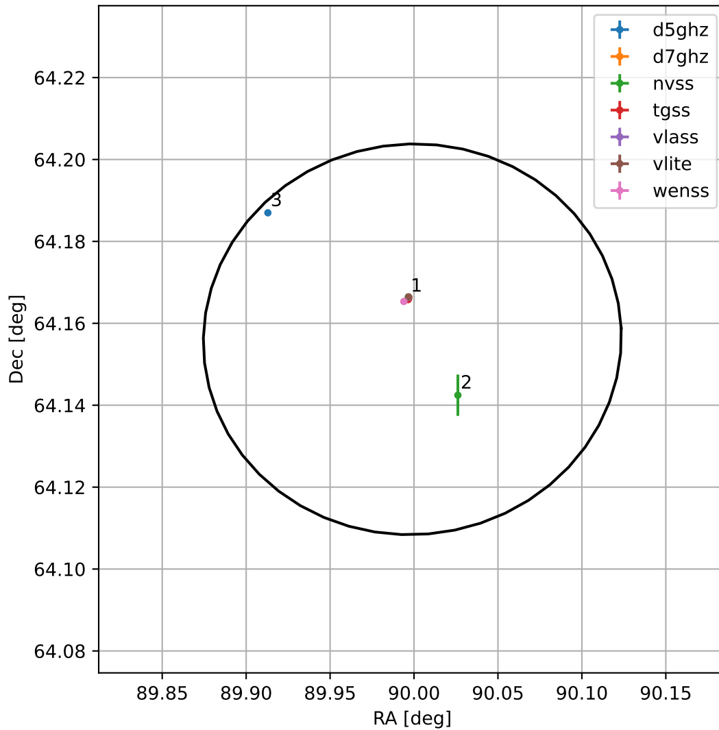
4FGL J0559.9+6409
