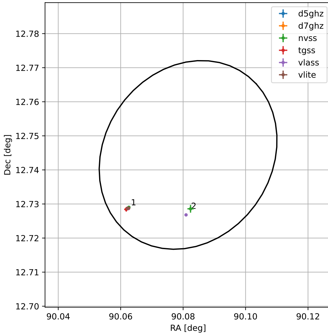
4FGL J0600.3+1244
