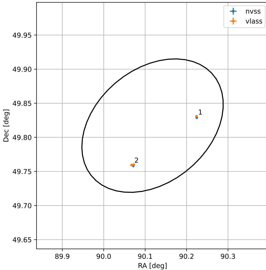
4FGL J0600.4+4949
