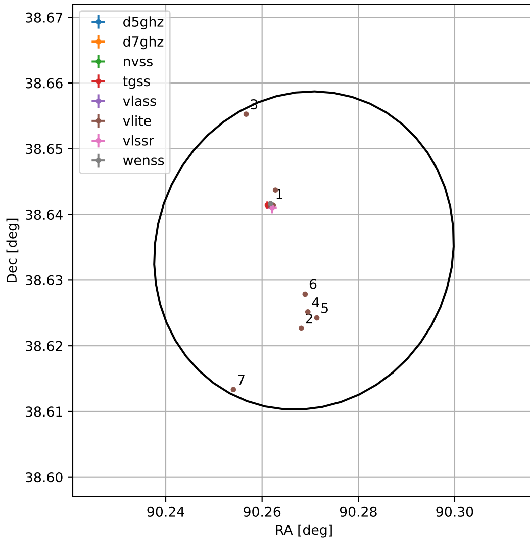
4FGL J0601.0+3838
