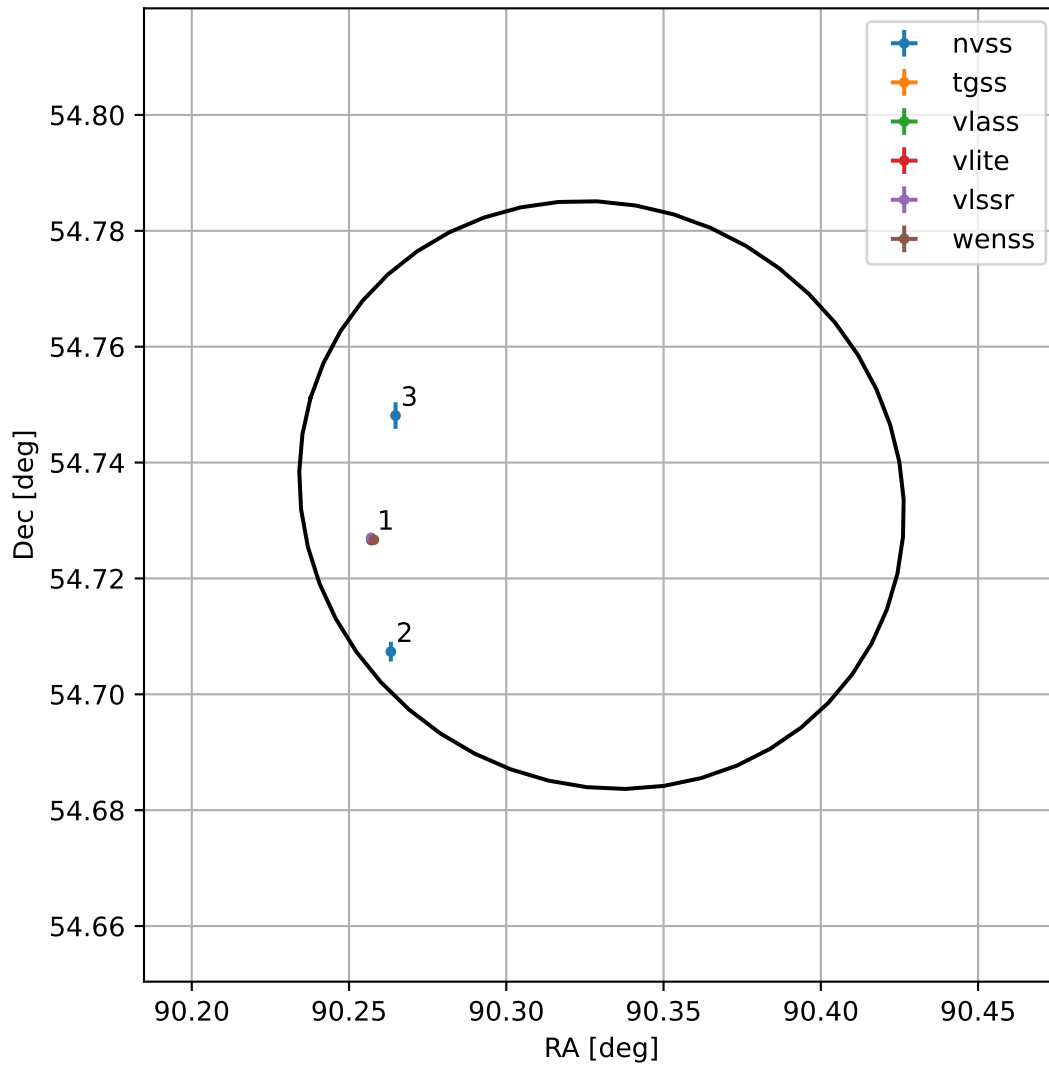
4FGL J0601.3+5444
