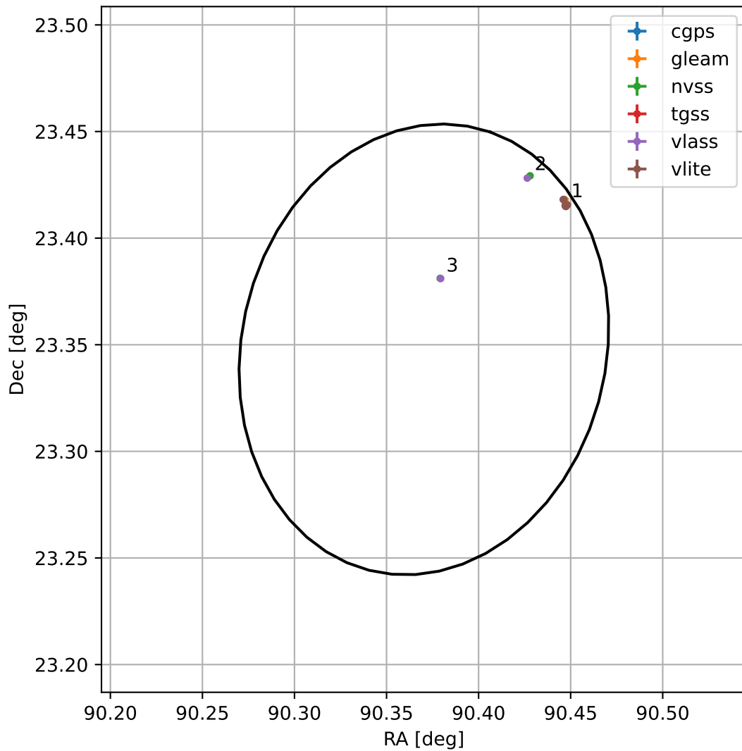
4FGL J0601.4+2320
