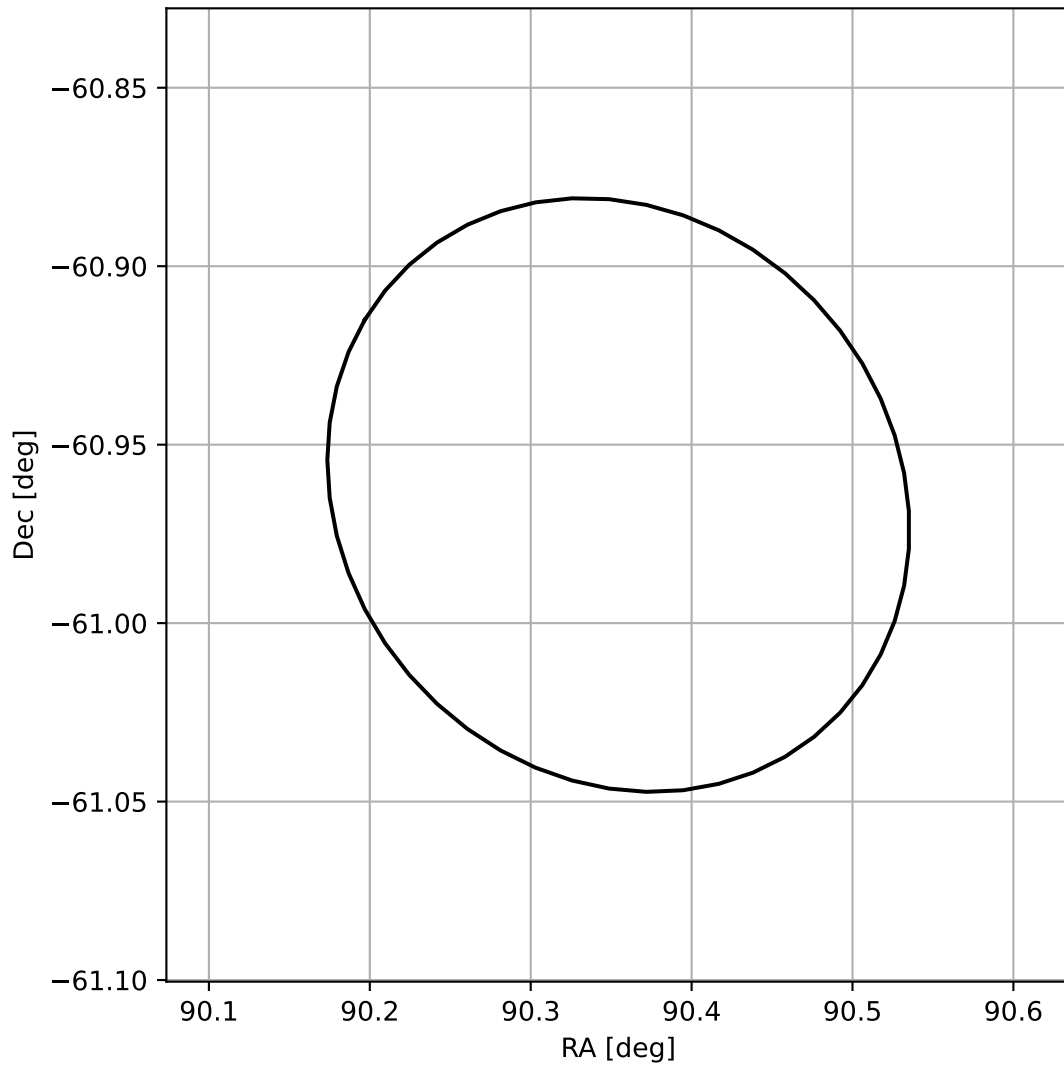
4FGL J0601.4-6057
