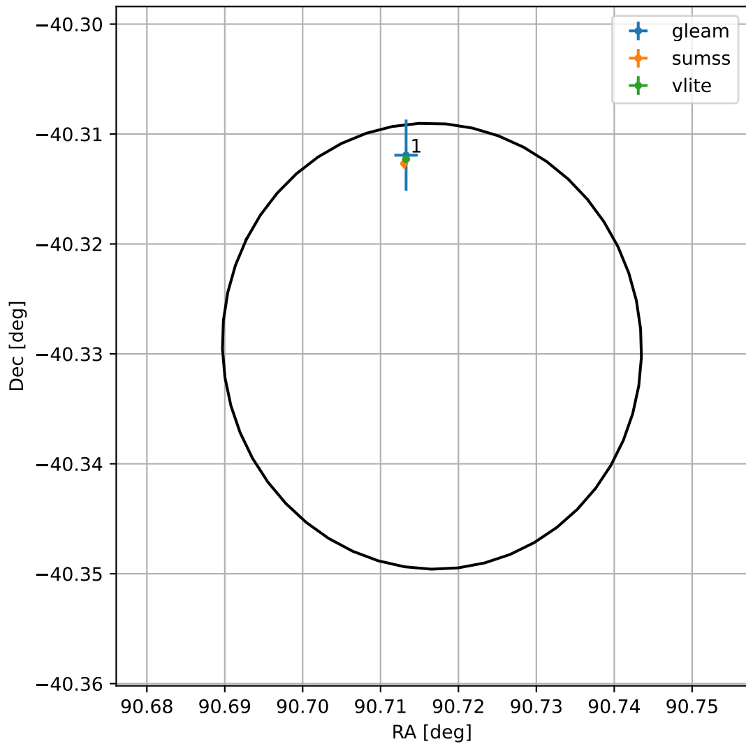
4FGL J0602.8-4019
