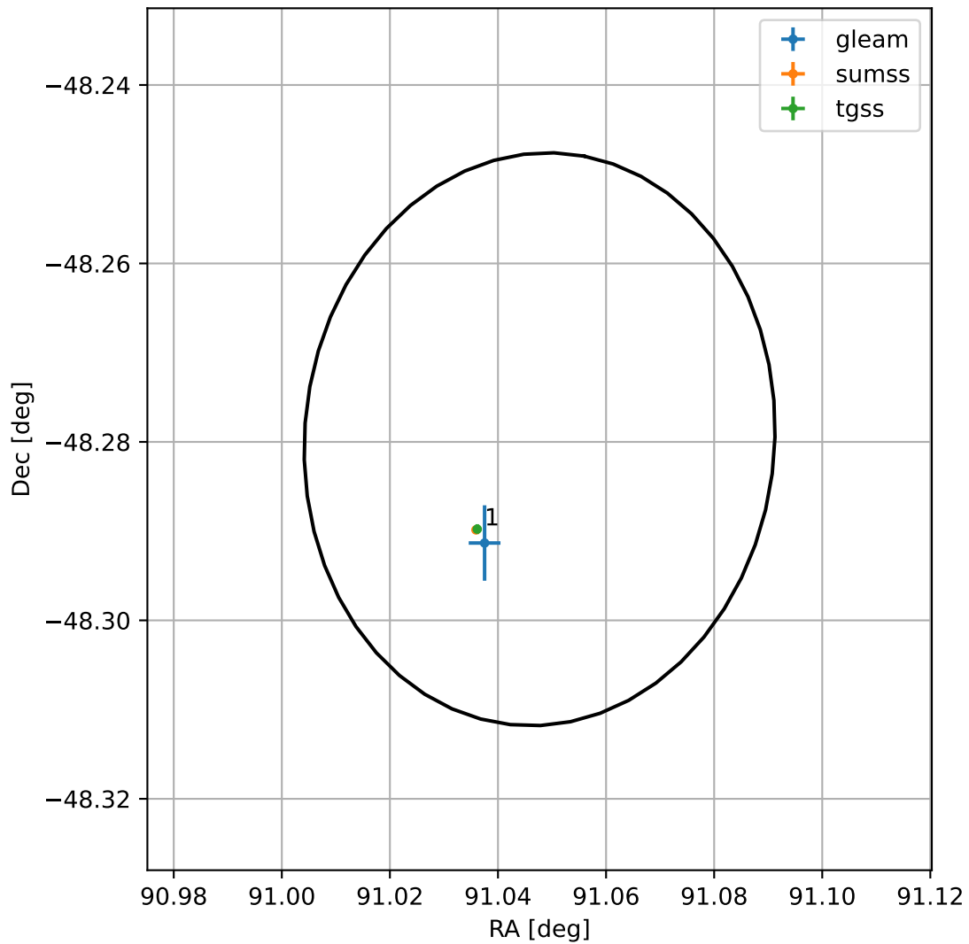
4FGL J0604.1-4816
