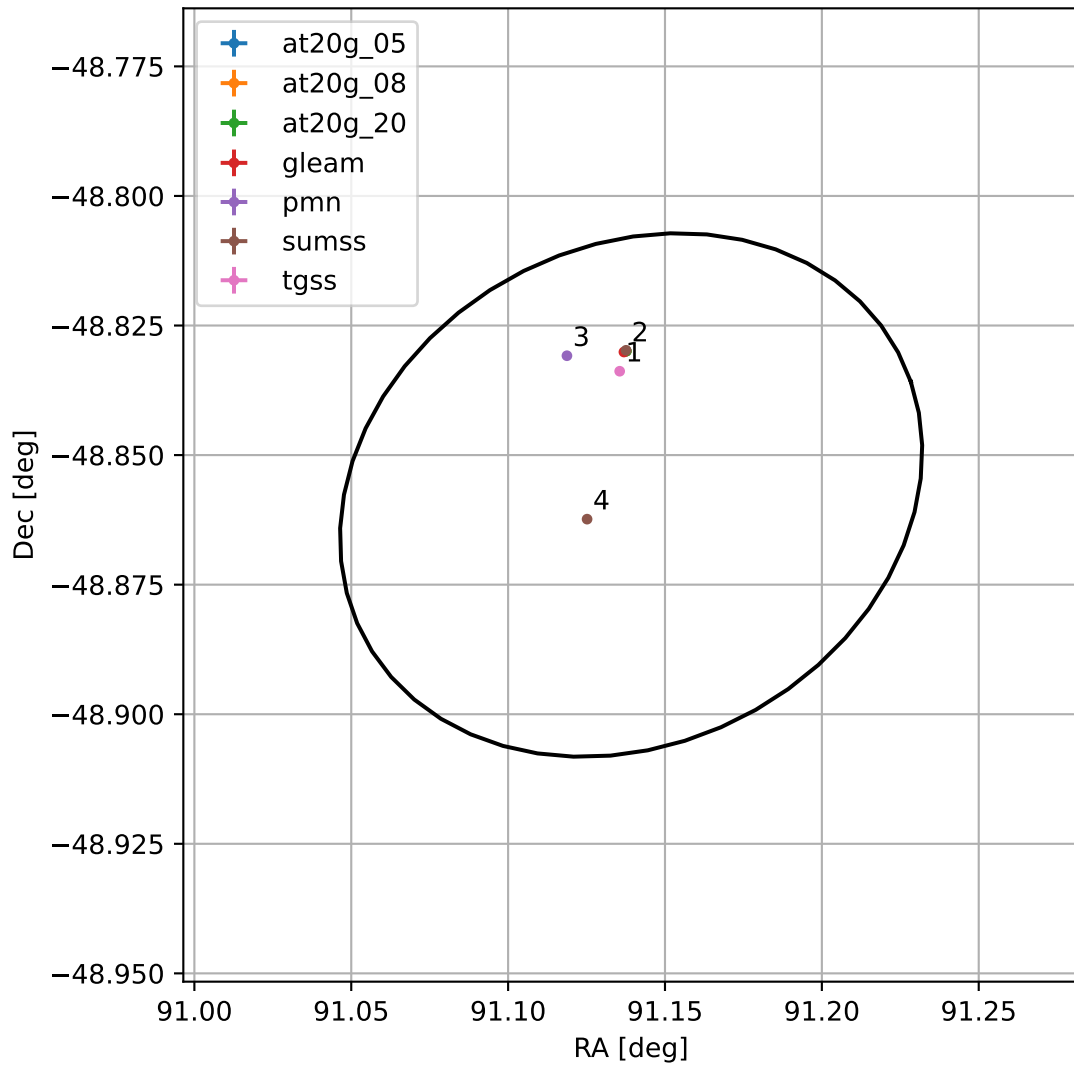
4FGL J0604.5-4851
