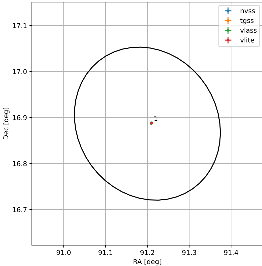
4FGL J0604.8+1653
