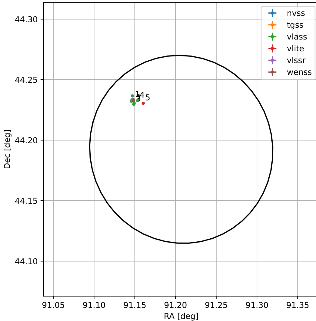
4FGL J0604.8+4411
