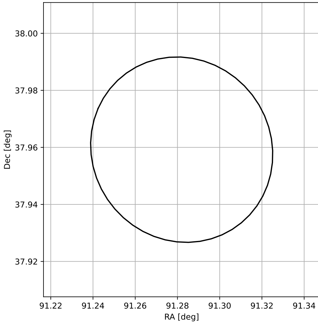
4FGL J0605.1+3757
