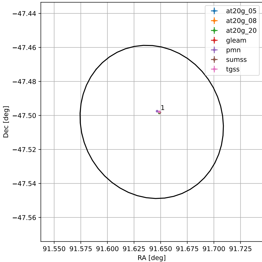
4FGL J0606.5-4730
