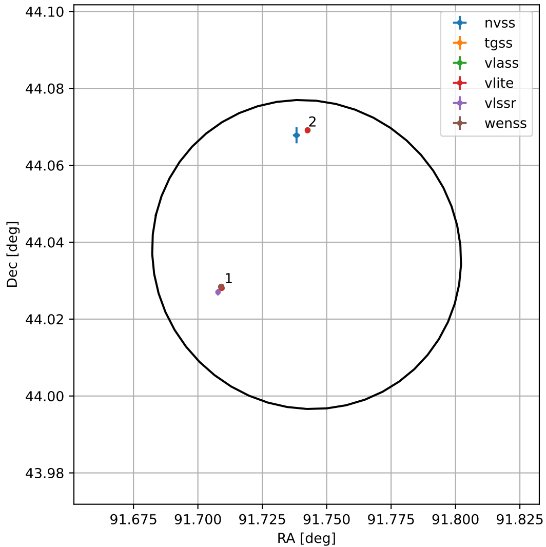
4FGL J0606.9+4402
