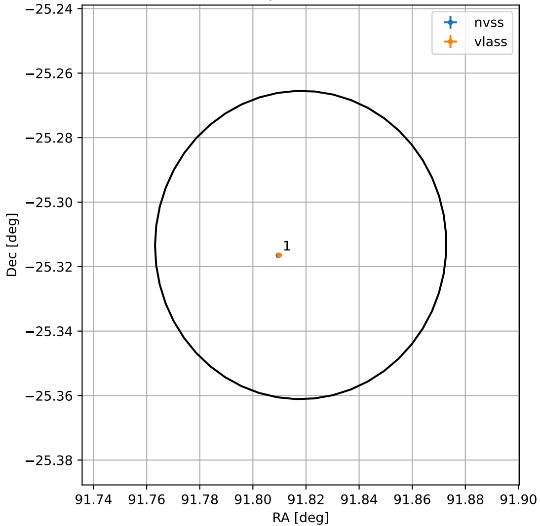
4FGL J0607.2-2518
