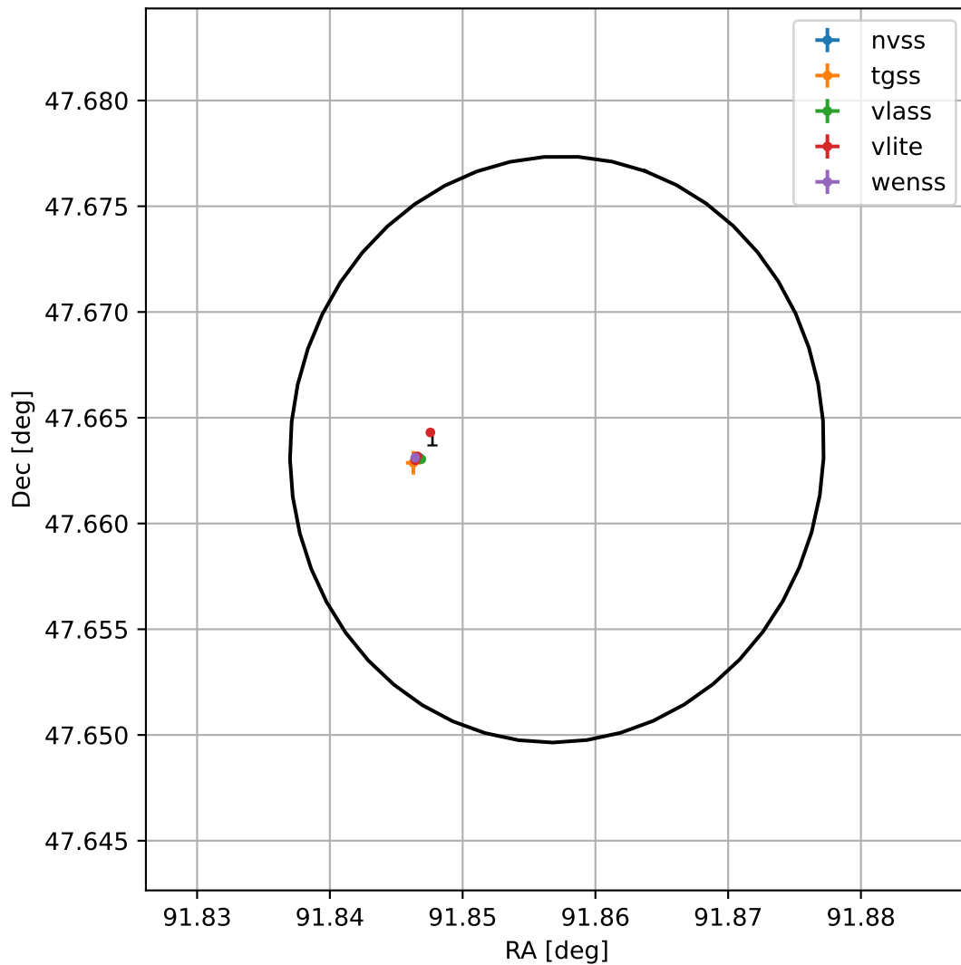
4FGL J0607.4+4739
