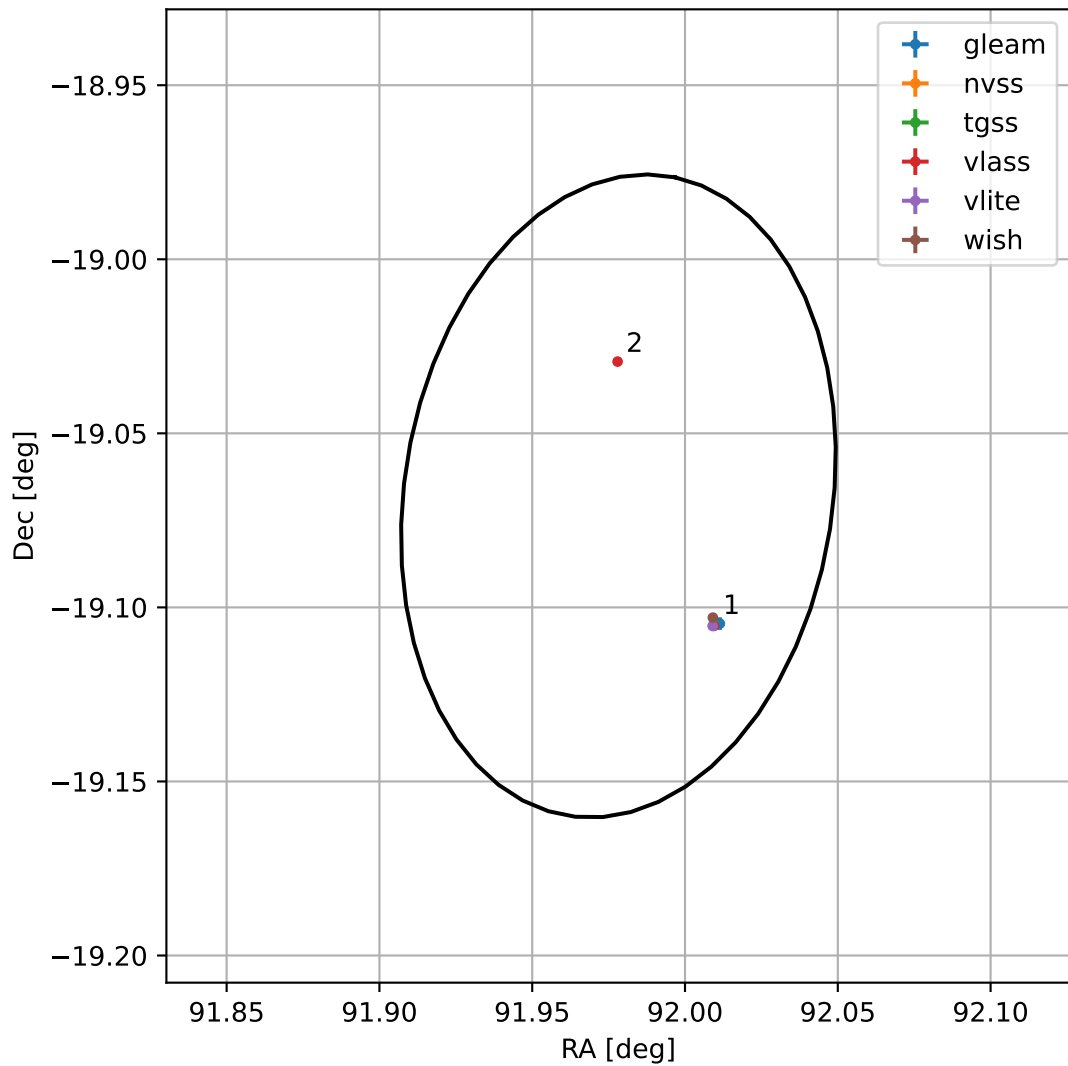
4FGL J0607.9-1904
