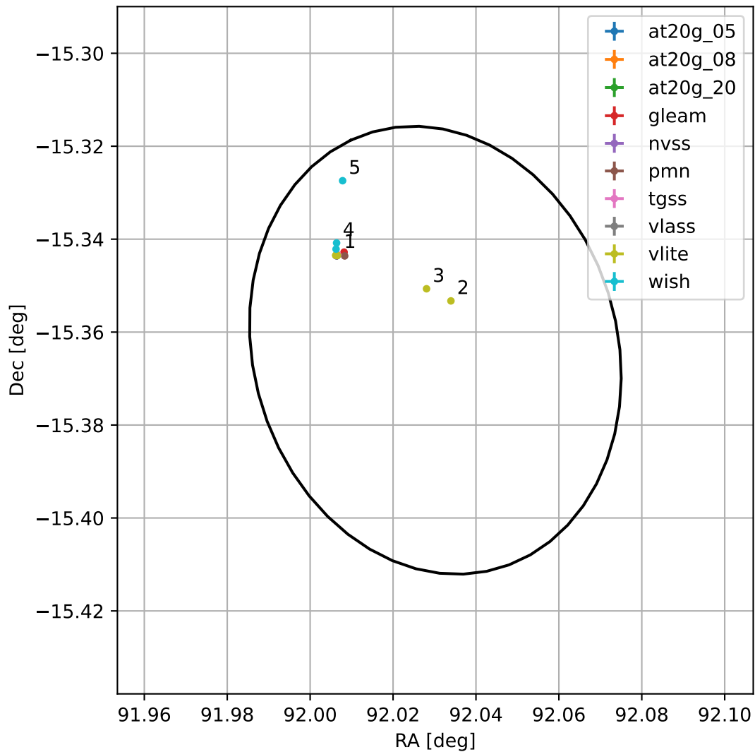
4FGL J0608.1-1521
