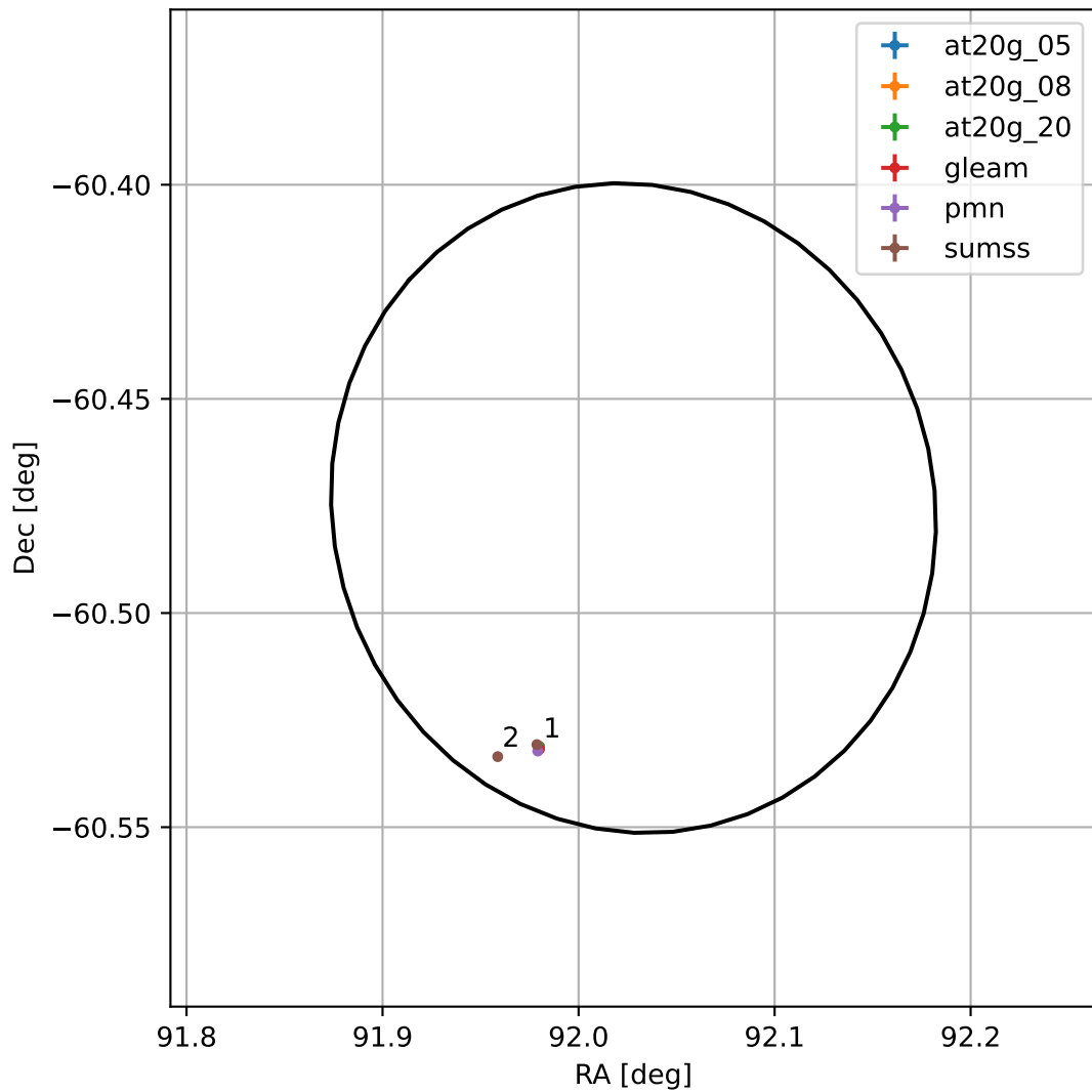
4FGL J0608.1-6028
