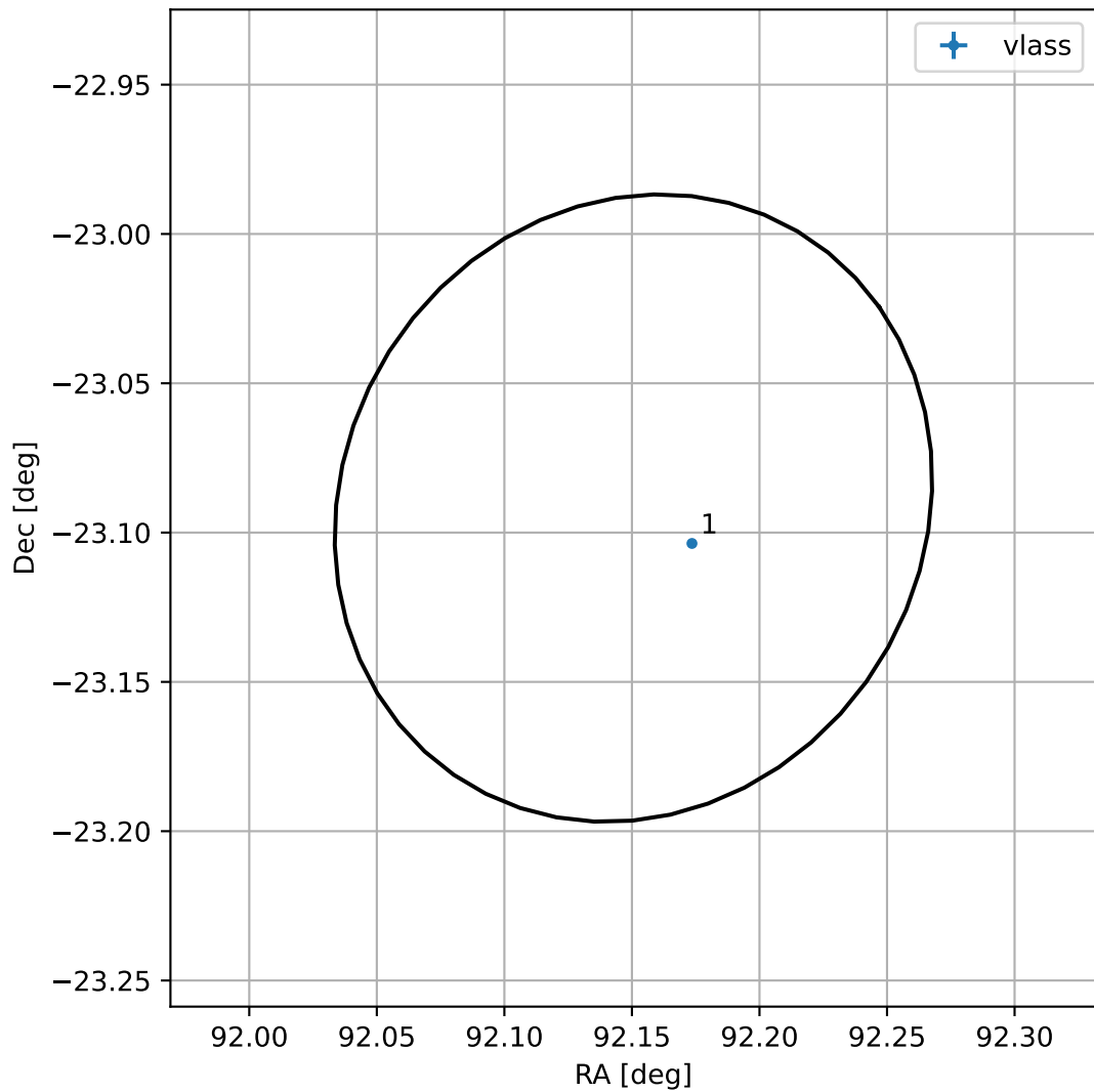
4FGL J0608.6-2305
