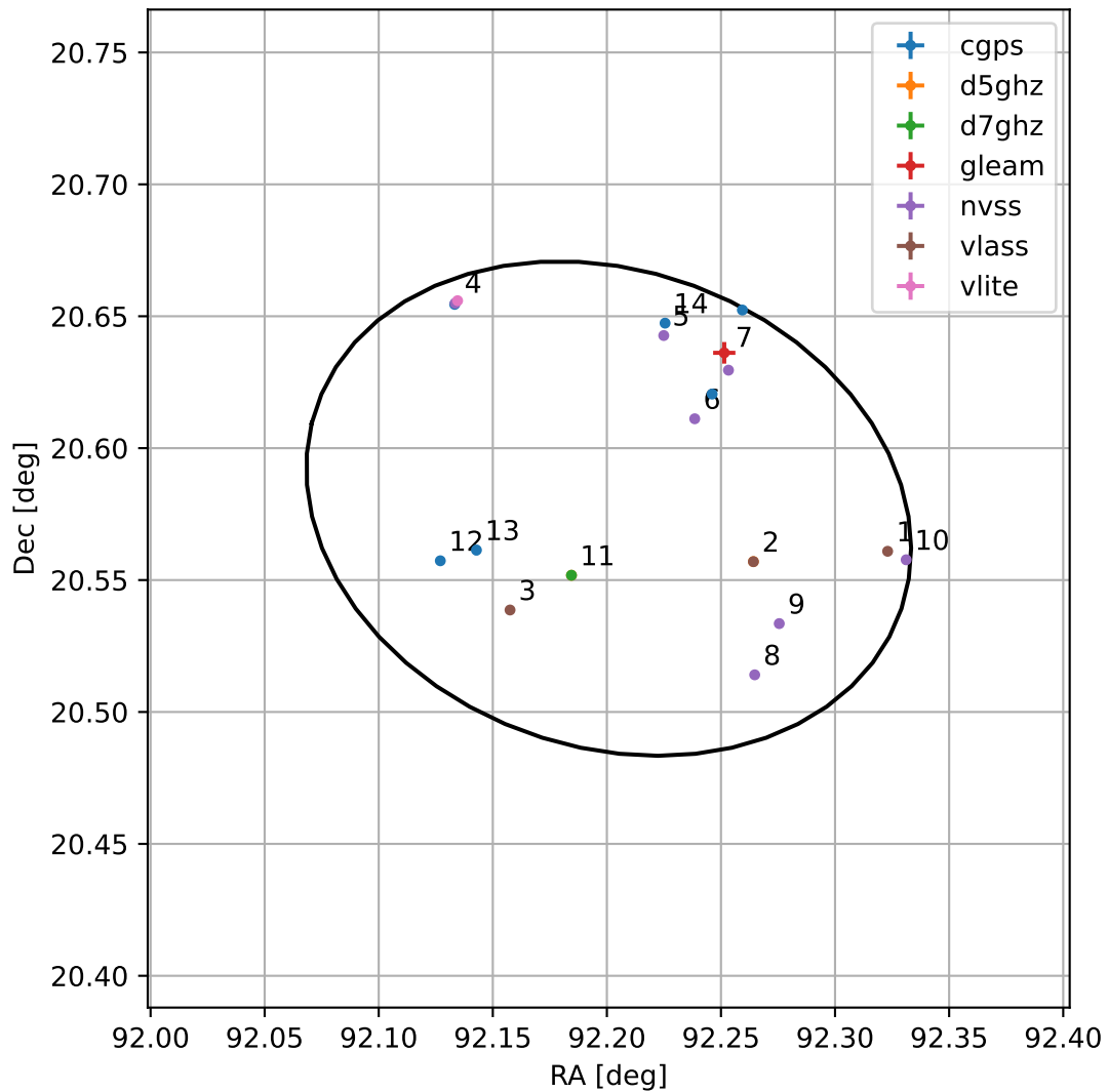
4FGL J0608.8+2034
