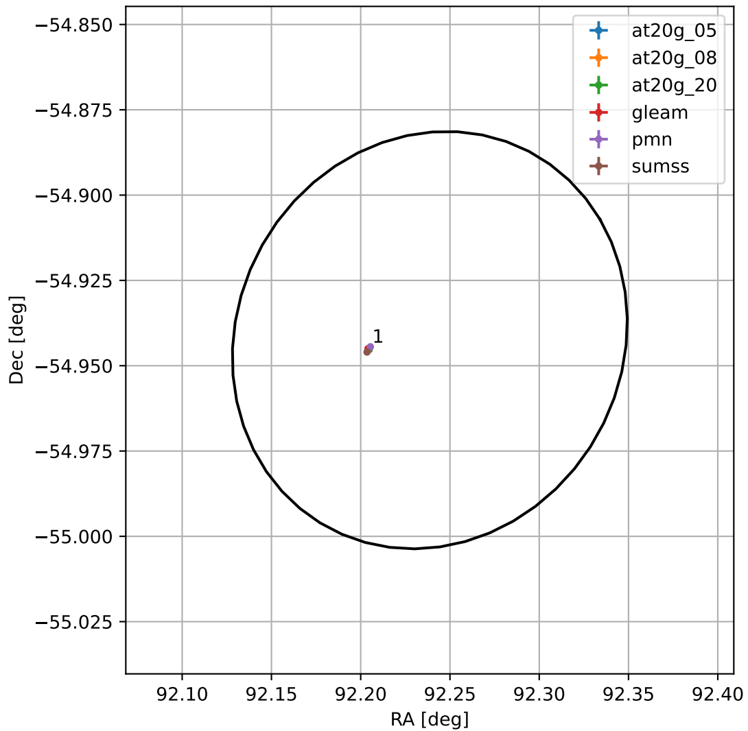
4FGL J0608.9-5456
