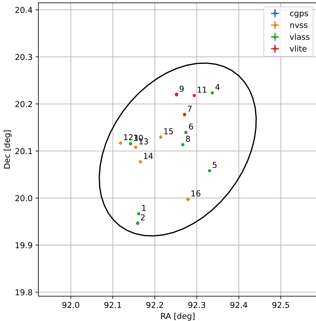
4FGL J0609.0+2006
