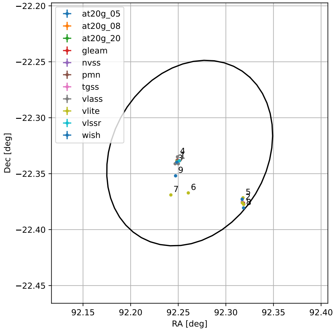
4FGL J0609.0-2219
