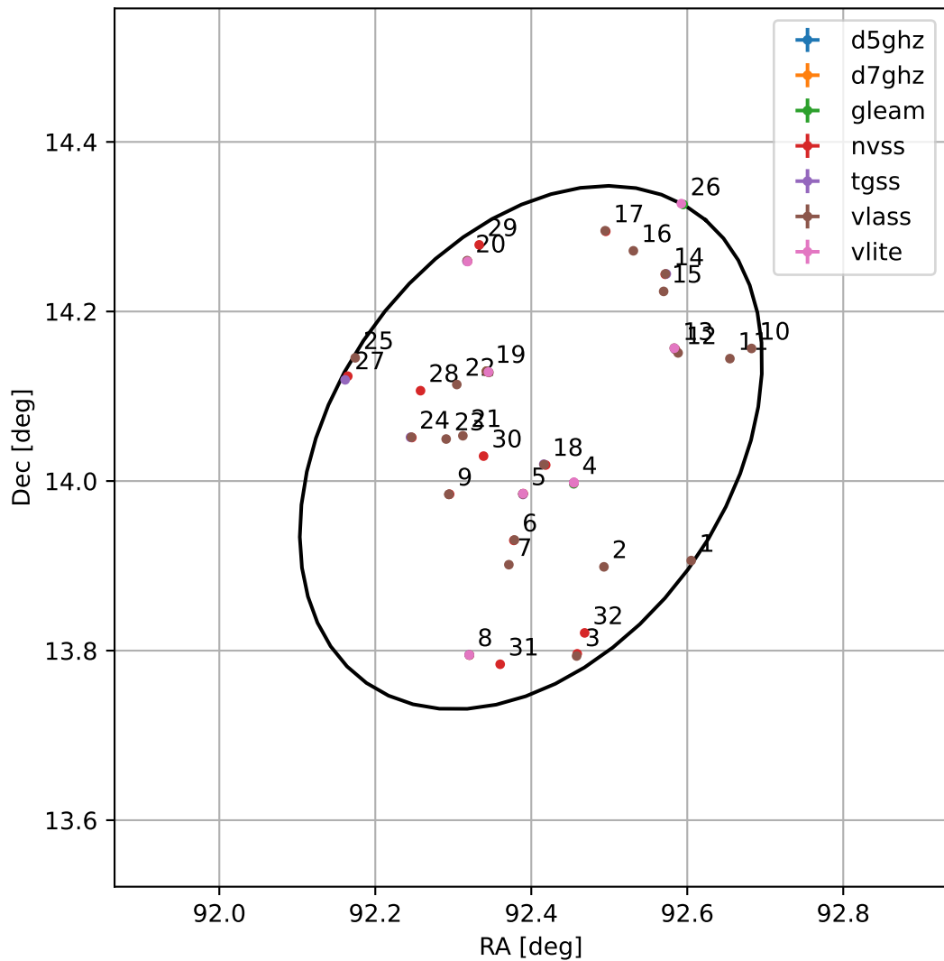
4FGL J0609.5+1402
