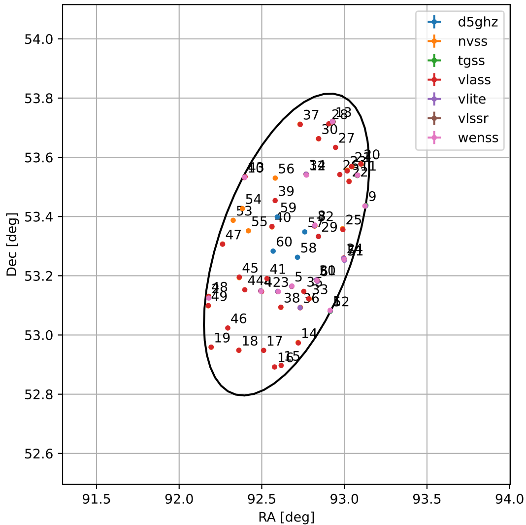
4FGL J0610.6+5318
