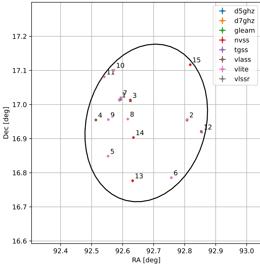
4FGL J0610.7+1656
